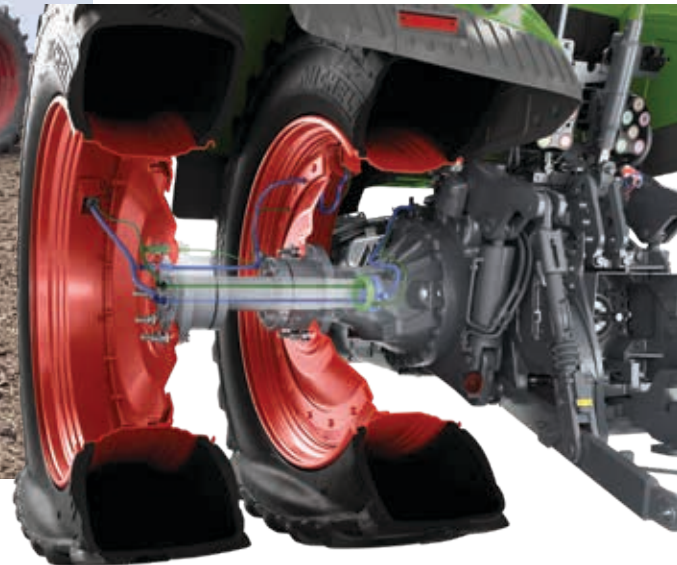
An onboard air compressor supplies air lines that are integrated into the wheel assembly. All components are secure and covered to prevent damage.
